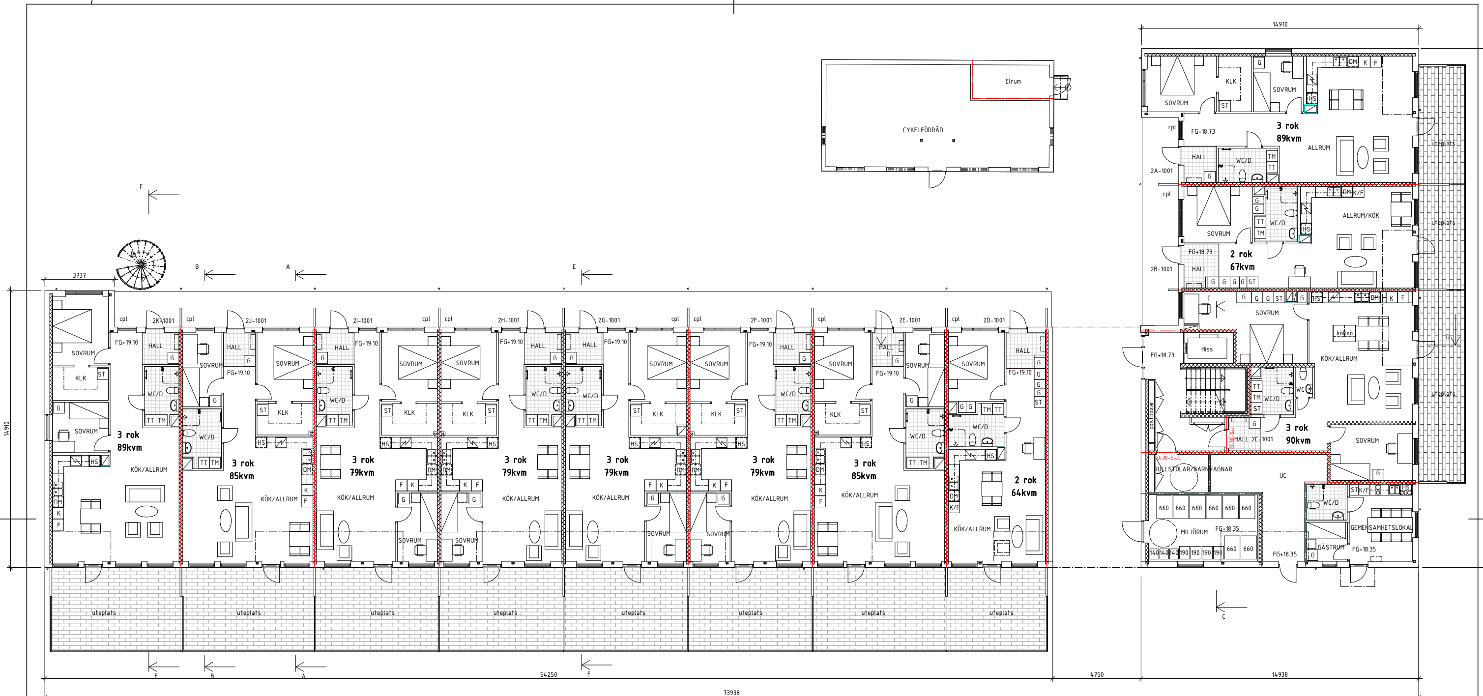
PLAN 1 1:100 (A3 1:200)
